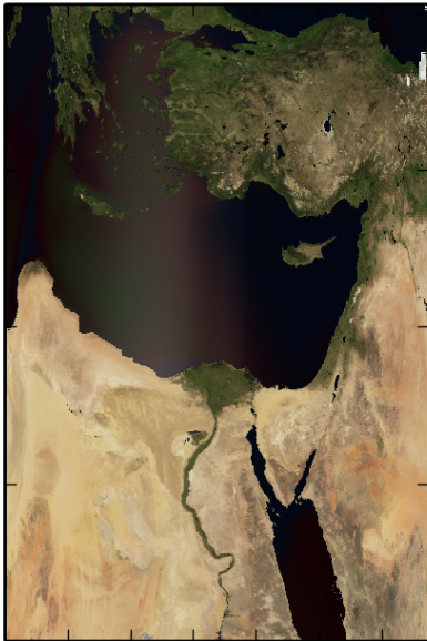
Albedo Only
