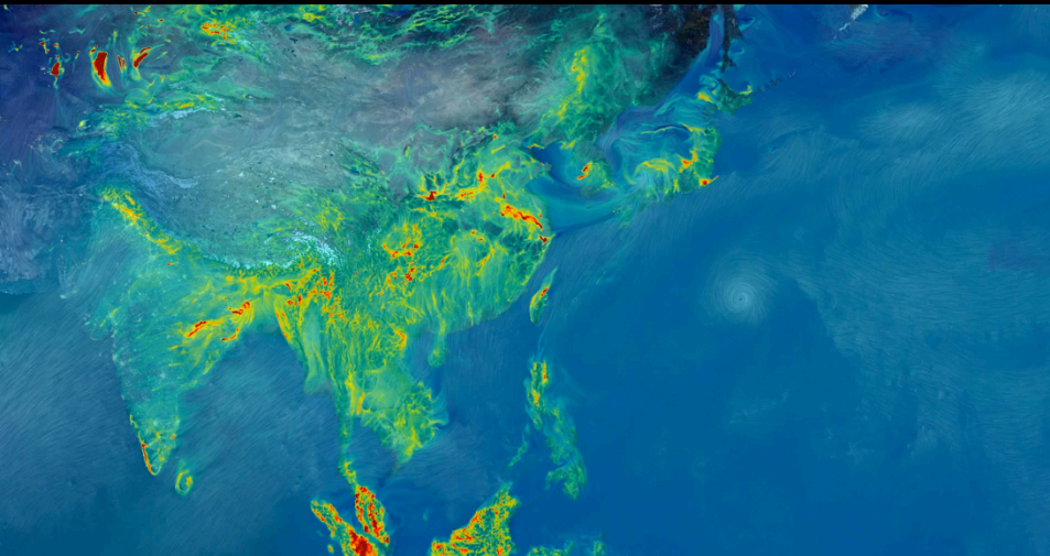
Surface CO 2 Concentration: The surface concentration of CO 2 highlights the fidelity of local emission centers and constituents being dispersed within the regional meso-scale flow.
