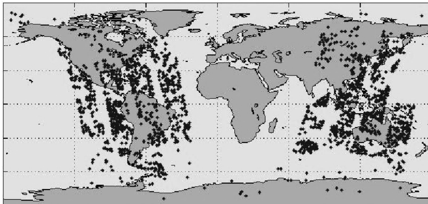
Simulated
