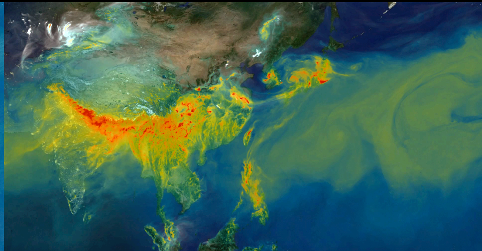
Column CO 2 Concentration: Surface emissions are lifted throughout the column and transported beyond the regional scales within the planetary flow.
