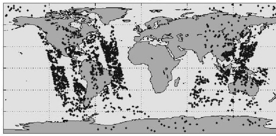
Real
