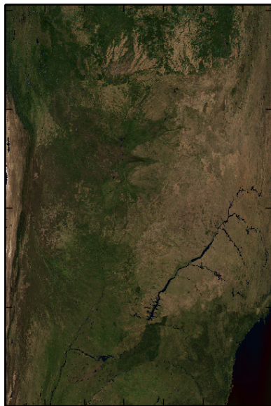
Albedo Only
