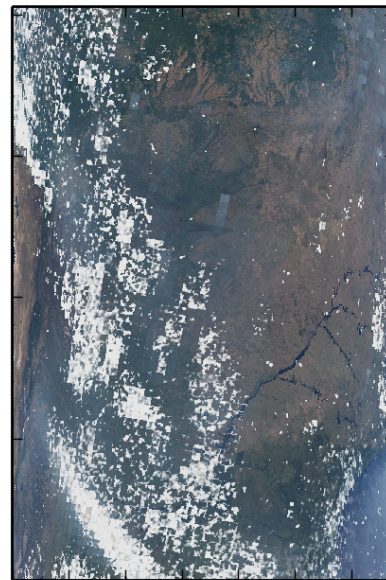
Everything
