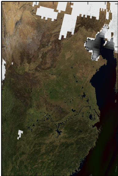
Albedo Only
